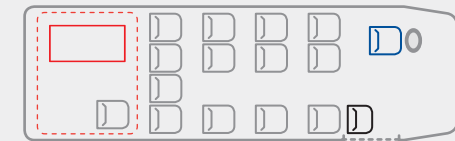
16/14 + 1 wheelchair space with 2 batteries
